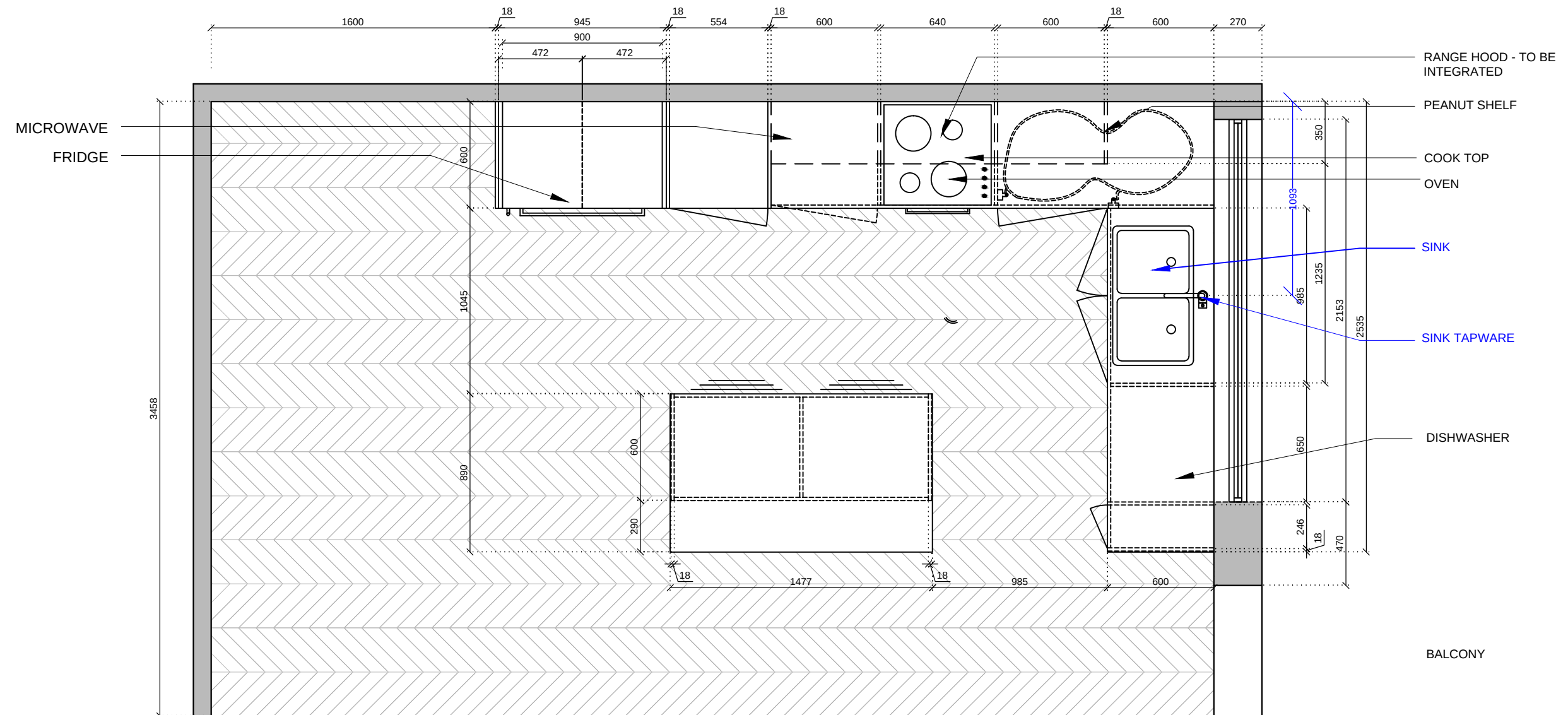
FLOOR AND PLUMBING PLAN
