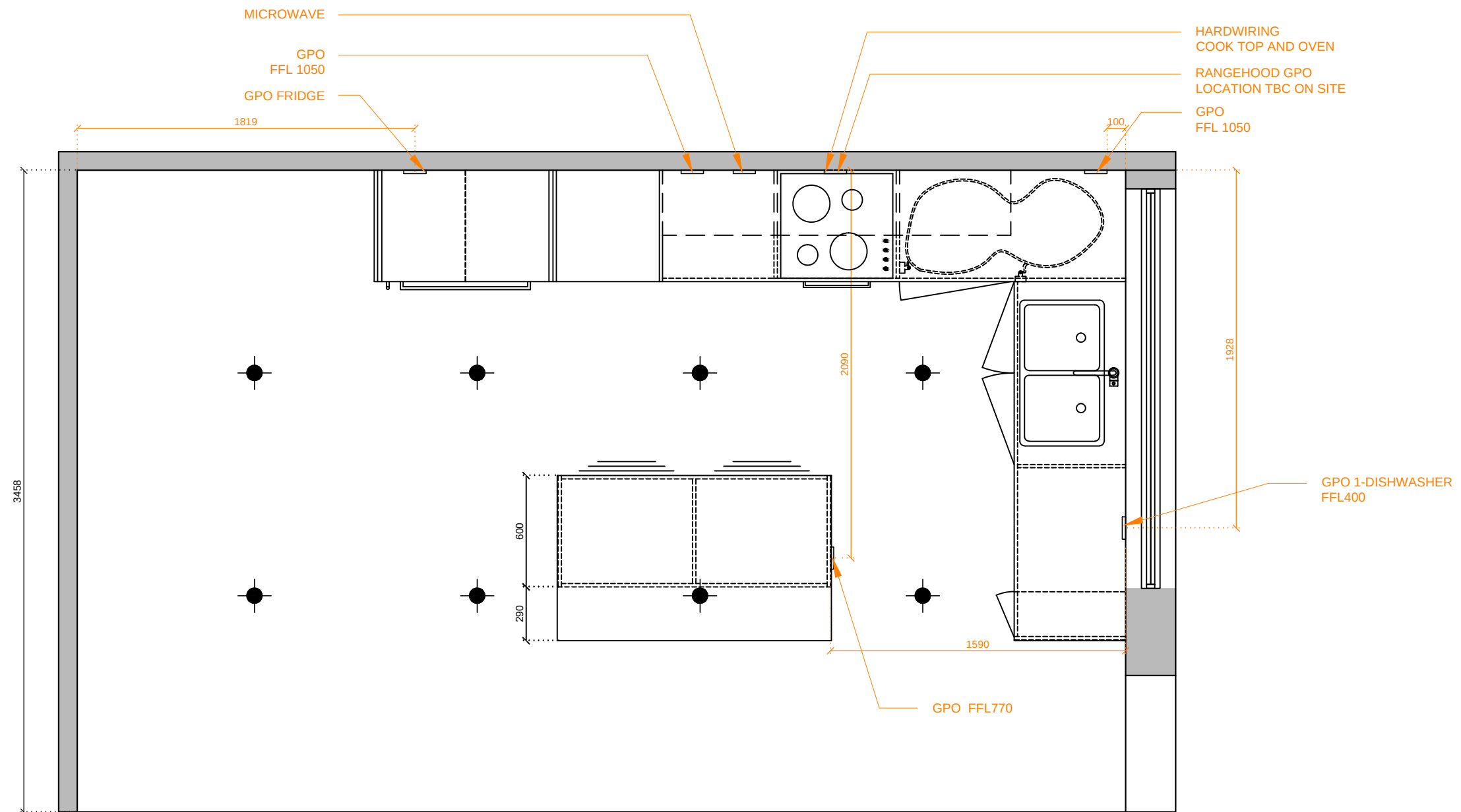
CEILING AND ELECTRICAL PLAN
